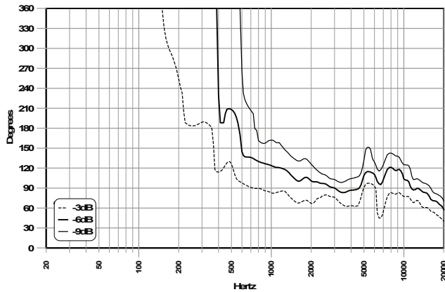
Vertical Beamwidth
