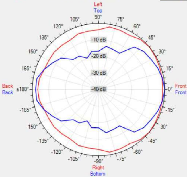
Data Shown: COLS41 (Apart Audio) Display Parameters: Frequency: 1000Hz (1/24th Octave)
