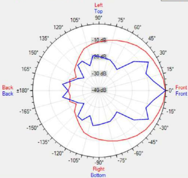
Data Shown: COLS41 (Apart Audio) Display Parameters: Frequency: 4000Hz (1/24th Octave)
