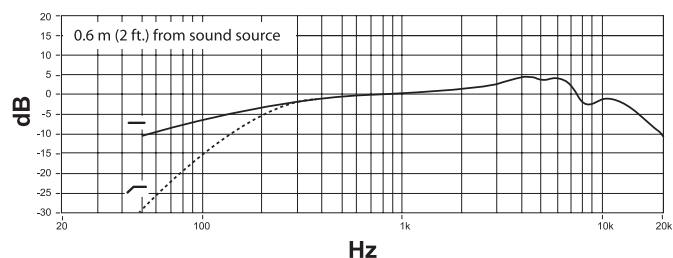
Frequency Response
