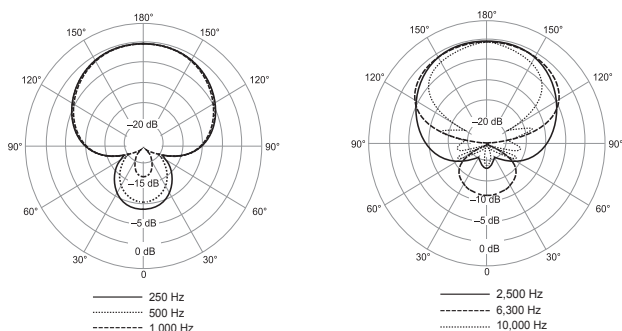
Polar Pattern
