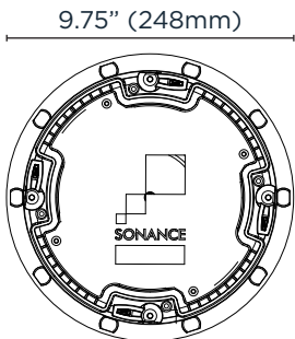
8.25" (210mm) VP66R SST/SUR Back View
