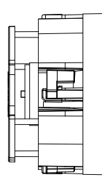
4.75" (121mm) VP62R SST/SUR Side View
