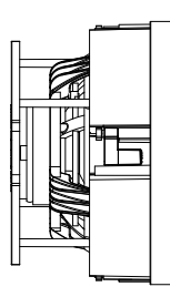
5.875" (149mm) VP86R SST/SUR Side View
