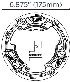
5.875" (149mm) VP46R SST/SUR Back View
