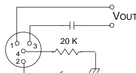
TEST CIRCUIT AND WIRING FIGURE 4
