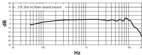
Frequency Response
