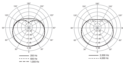
Polar Pattern
